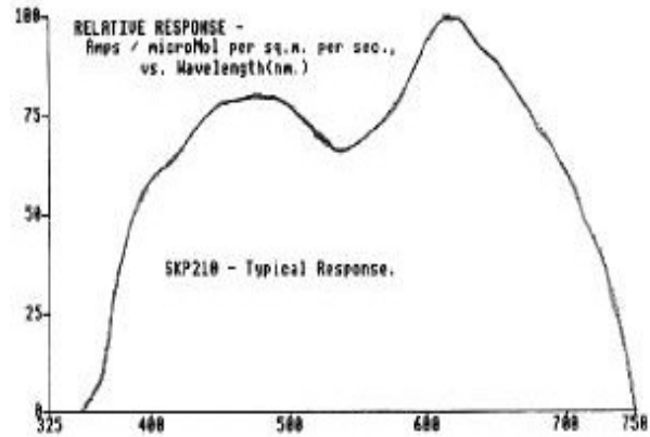
PAR-«special»-Sensor SKP210
